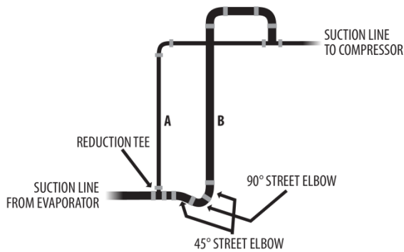
Figure 9 - Double Suction Riser Construction
