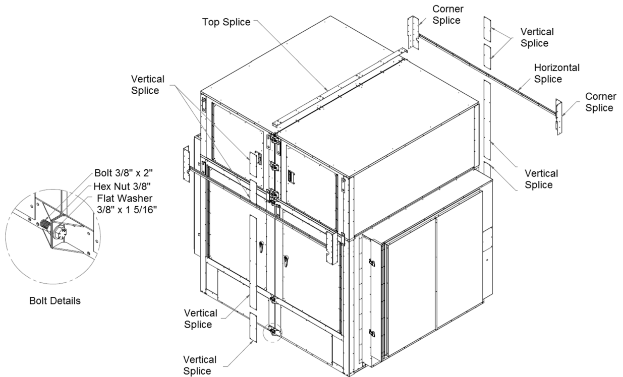
Figure 9 - Dual Unit Assembly Details
