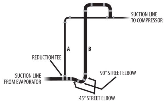
Figure 9 - Double Suction Riser Construction
