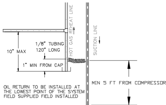
Figure 12 - Oil Return Line
