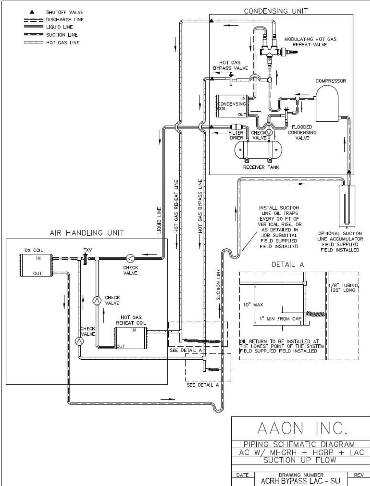
Figure 32 - A/C with Modulating Hot Gas Reheat and Hot Gas Bypass + LAC Split System Piping, Suction Up
