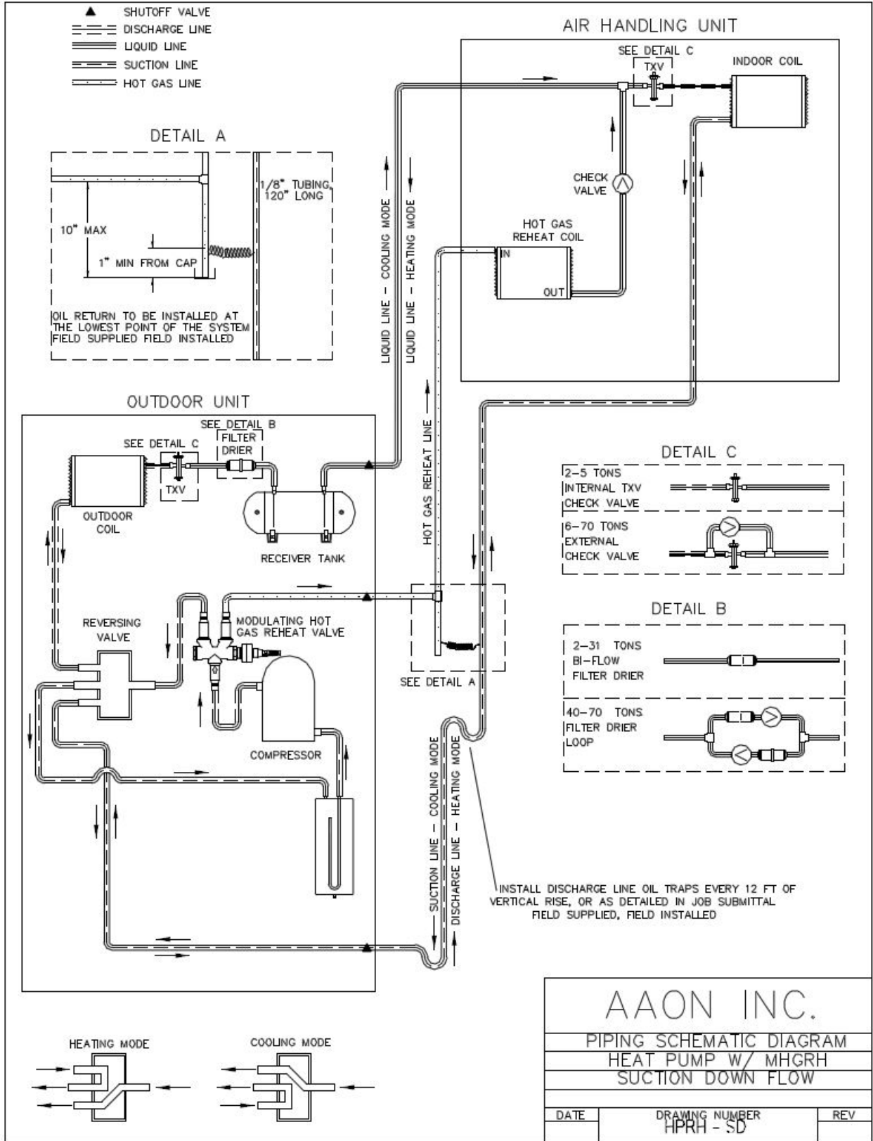
Figure 35 - Heat Pump with Modulating Hot Gas Reheat Split System Piping, Suction Down
