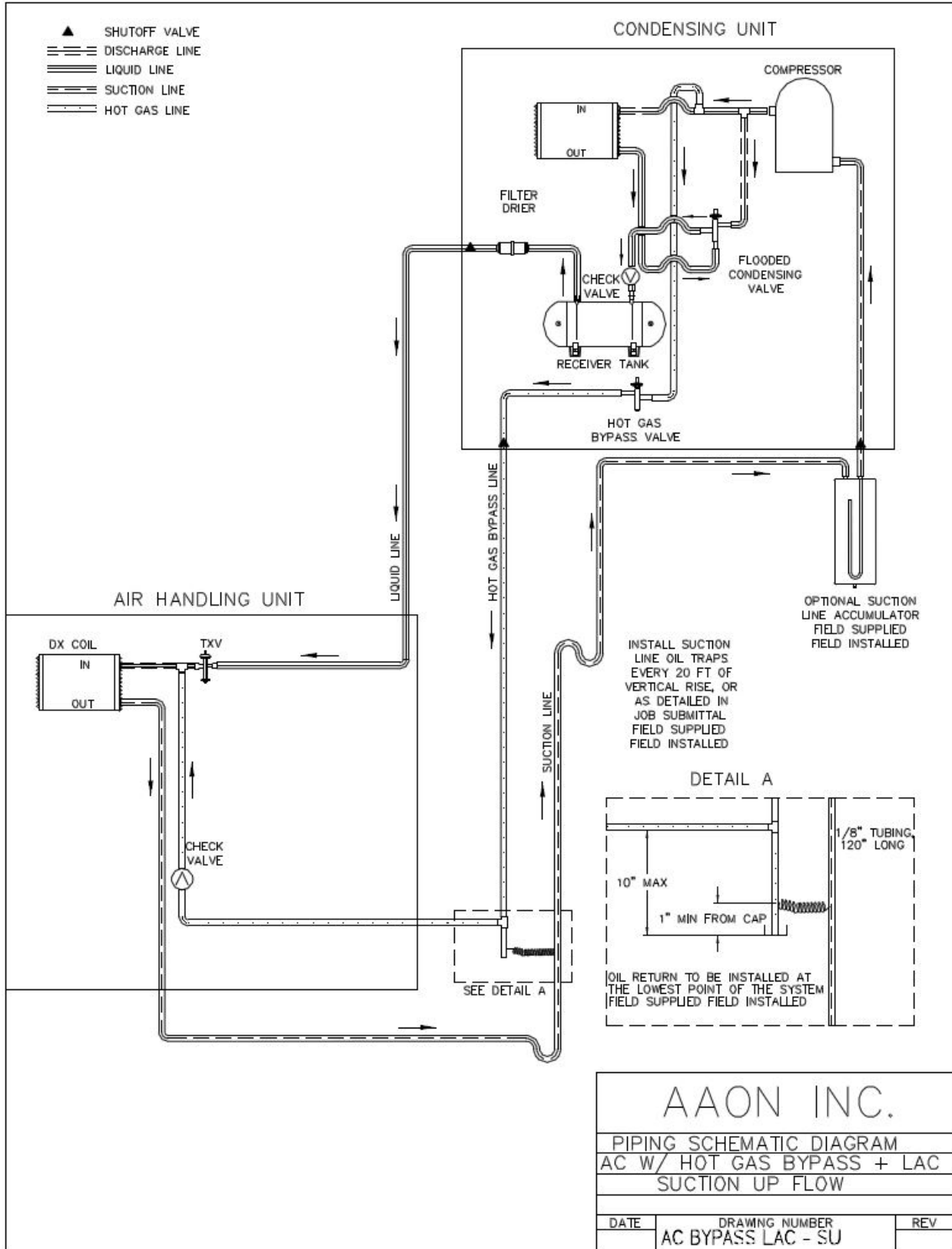
Figure 28 - A/C with Hot Gas Bypass + LAC Split System Piping, Suction Up
