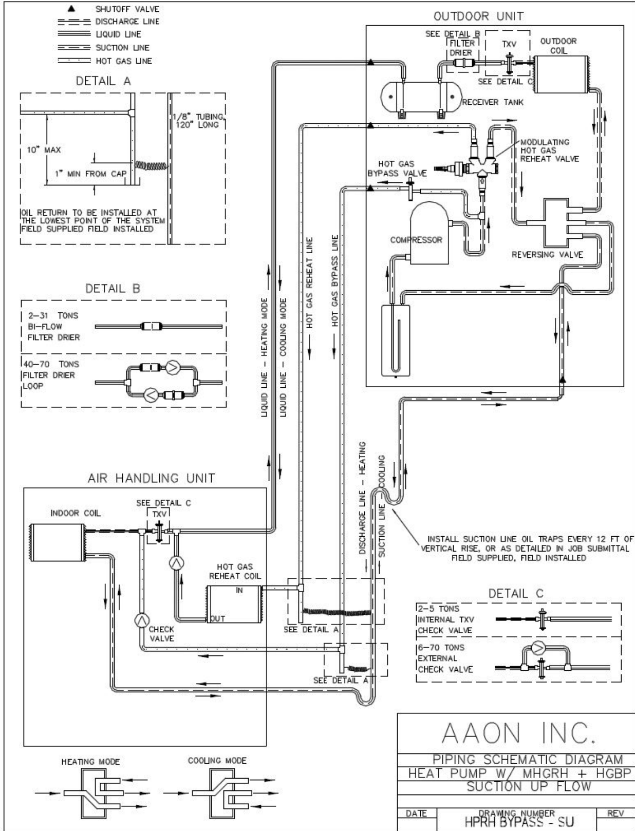
Figure 40 - Heat Pump with Modulating Hot Gas Reheat and Hot Gas Bypass Split System Piping, Suction Up
