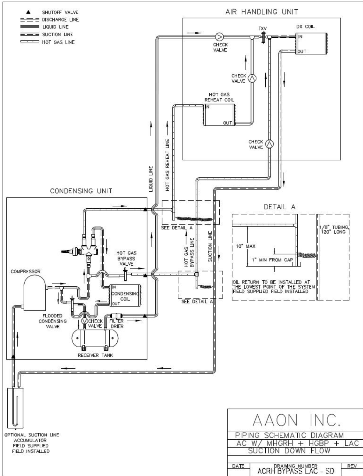
Figure 31 - A/C with Modulating Hot Gas Reheat and Hot Gas Bypass + LAC Split System Piping, Suction Down
