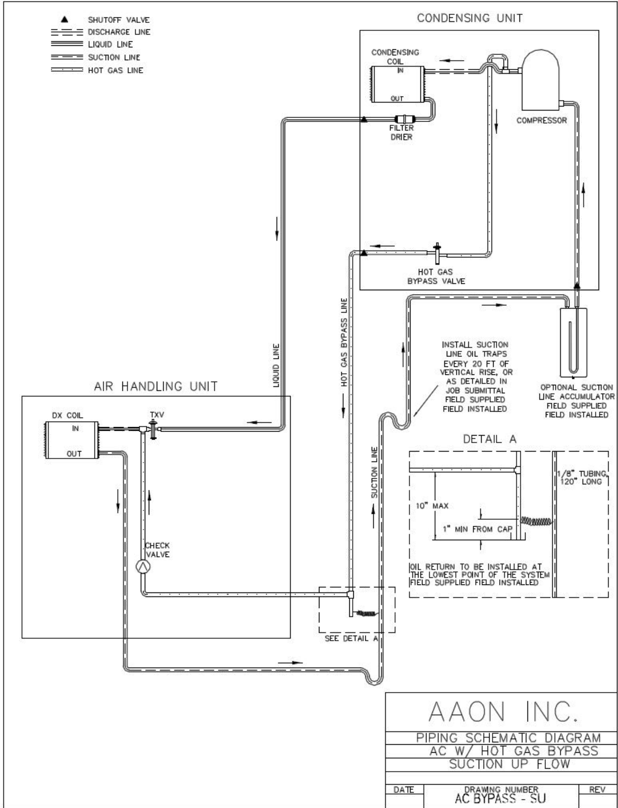
Figure 26 - A/C with Hot Gas Bypass Split System Piping, Suction Up
