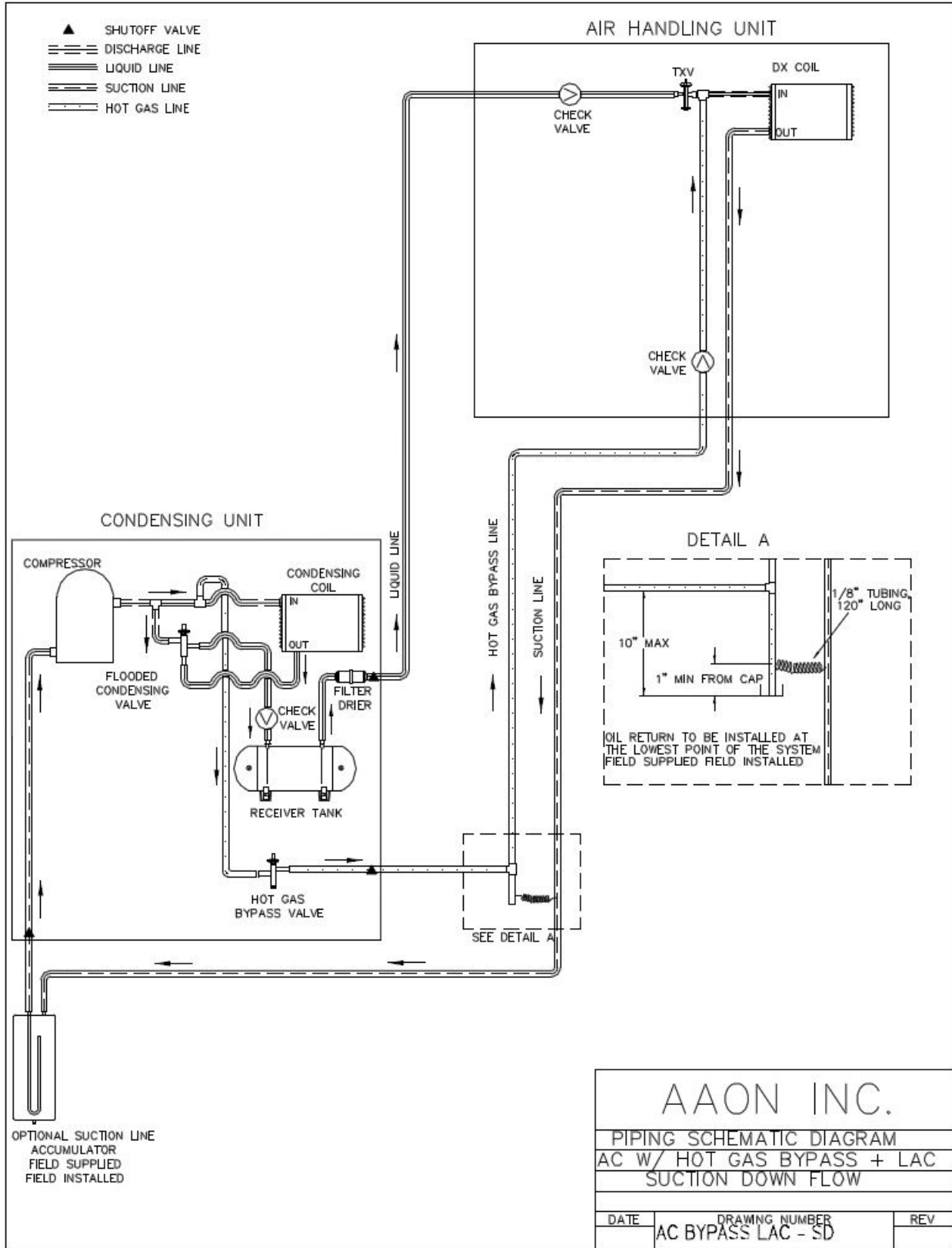
Figure 27 - A/C with Hot Gas Bypass + LAC Split System Piping, Suction Down
