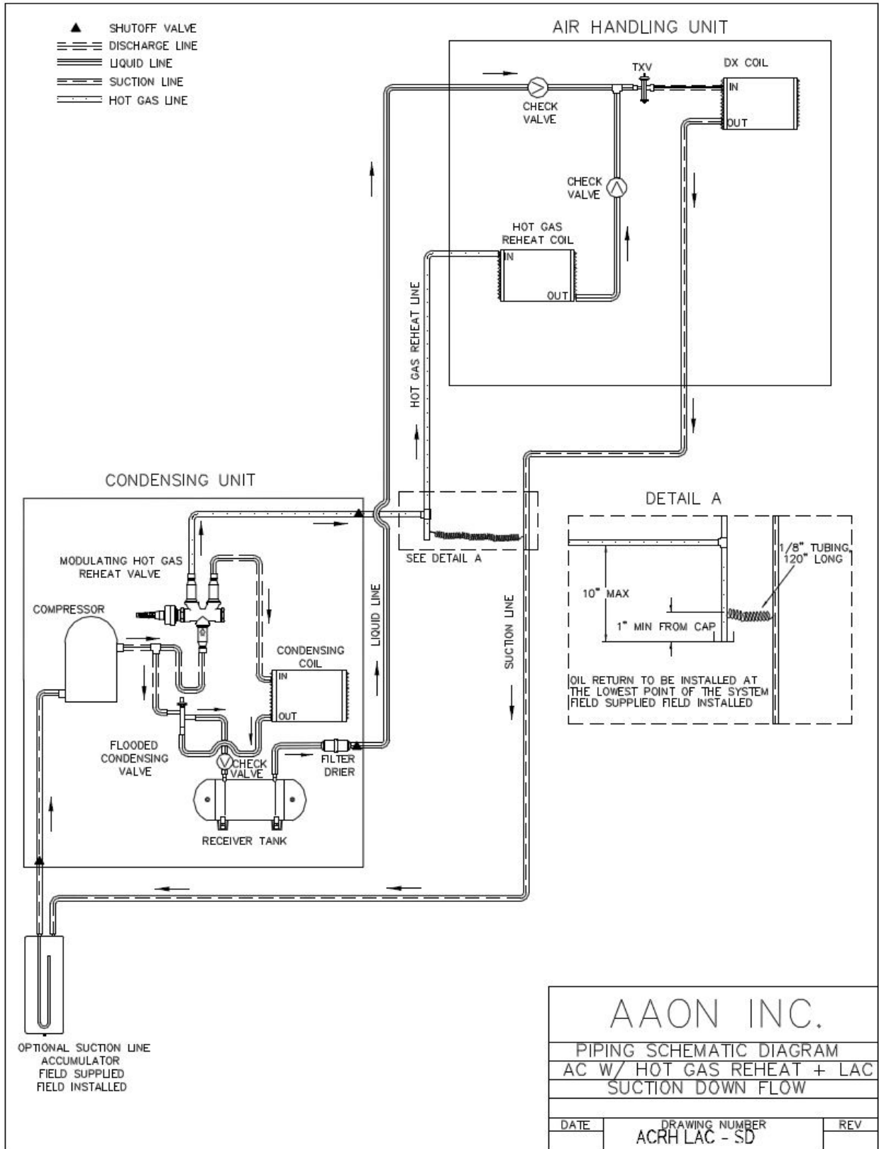
Figure 23 - A/C with Modulating Hot Gas Reheat Split + LAC System Piping, Suction Down
