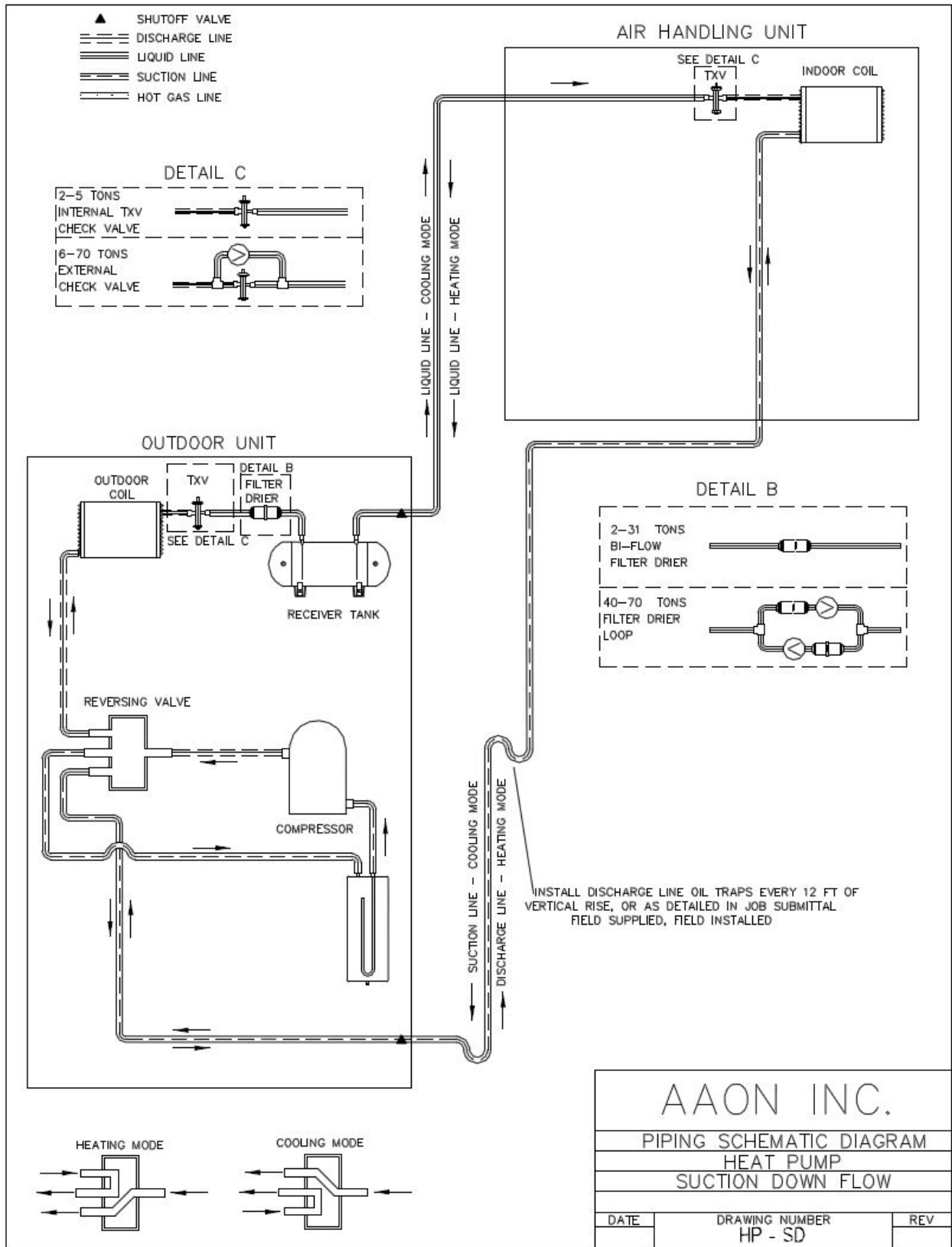
Figure 33 - Heat Pump Split System Piping, Suction Down
