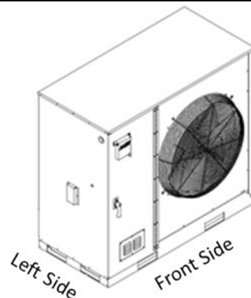
Figure 4 - Orientation of Series 2-7 ton Condensing Unit
