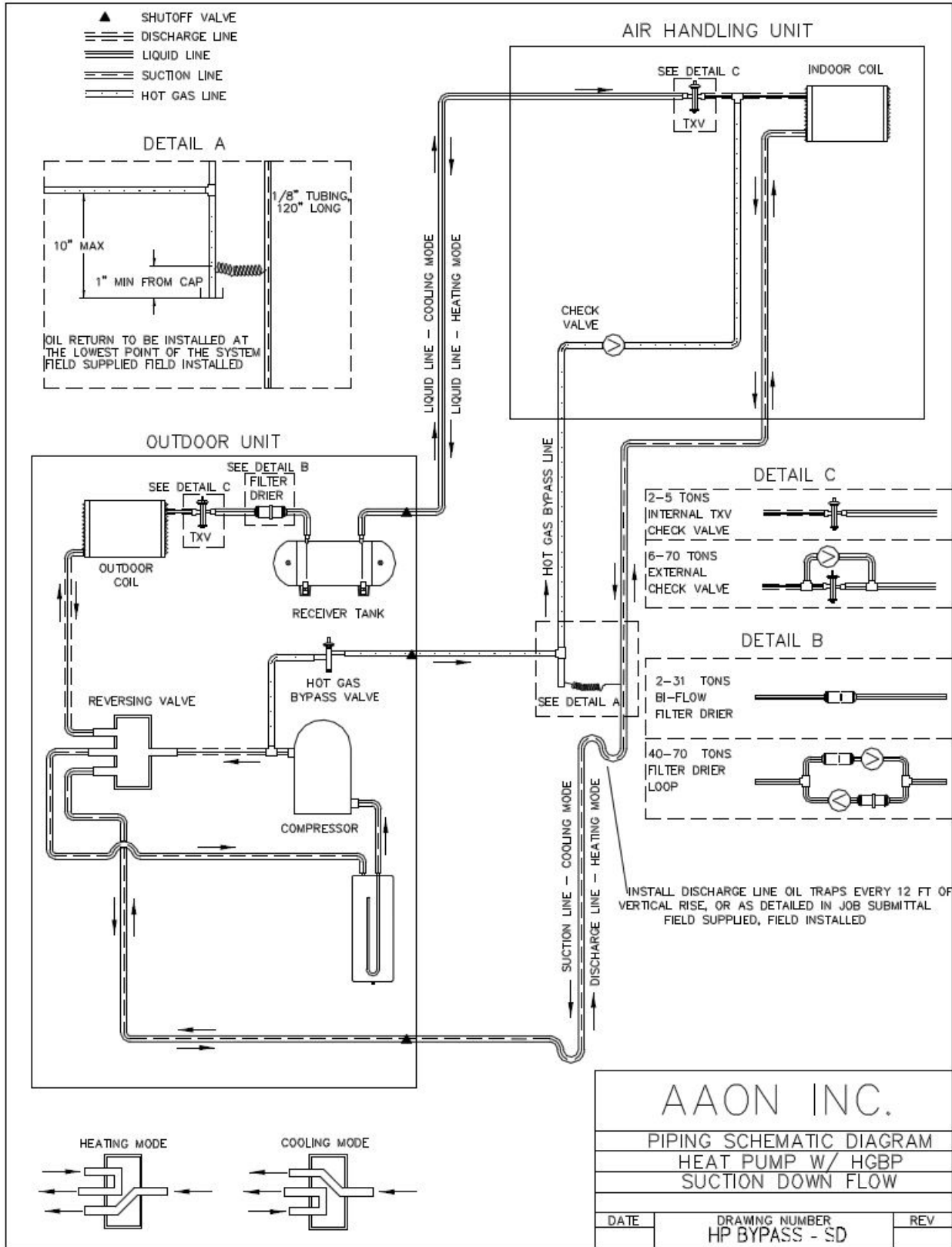
Figure 37 - Heat Pump with Hot Gas Bypass Split System Piping, Suction Down
