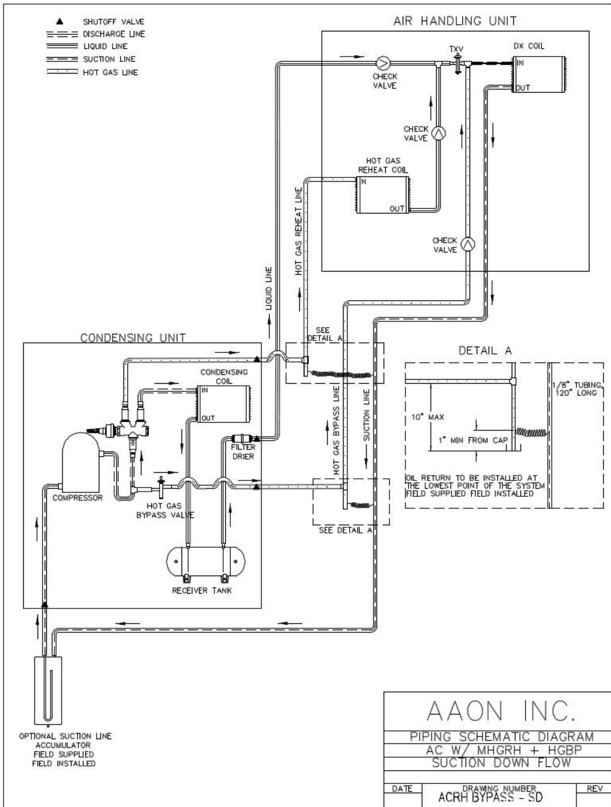
Figure 29 - A/C with Modulating Hot Gas Reheat and Hot Gas Bypass Split System Piping, Suction Down
