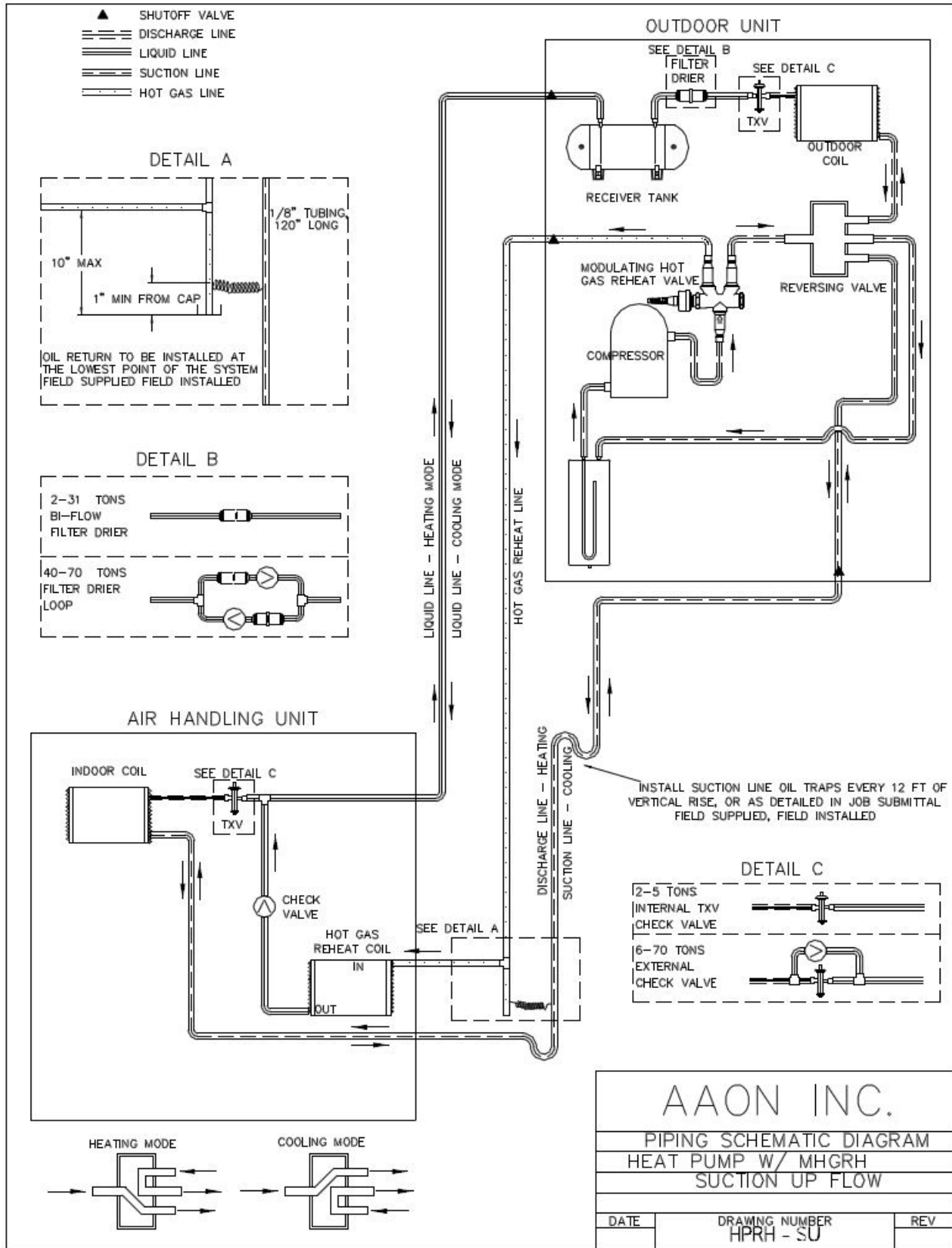
Figure 36 - Heat Pump with Modulating Hot Gas Reheat Split System Piping, Suction Up
