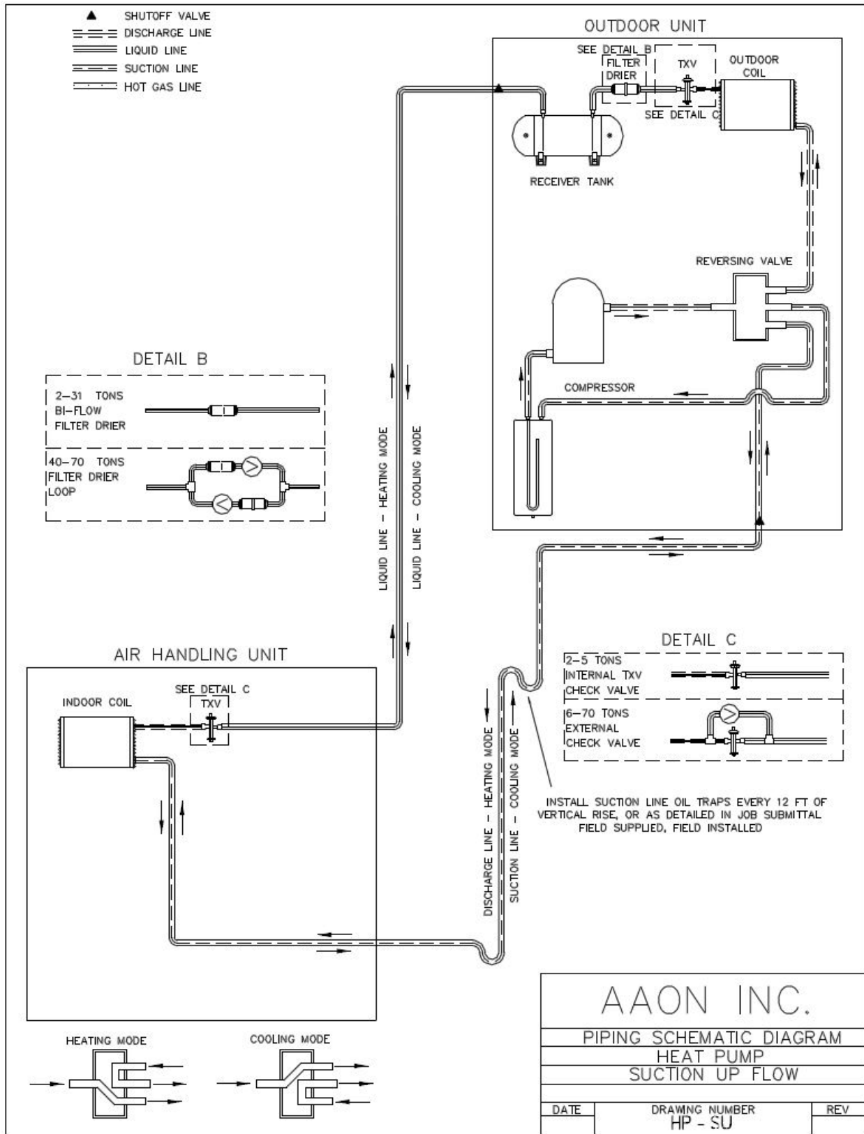
Figure 34 - Heat Pump Split System Piping, Suction Up
