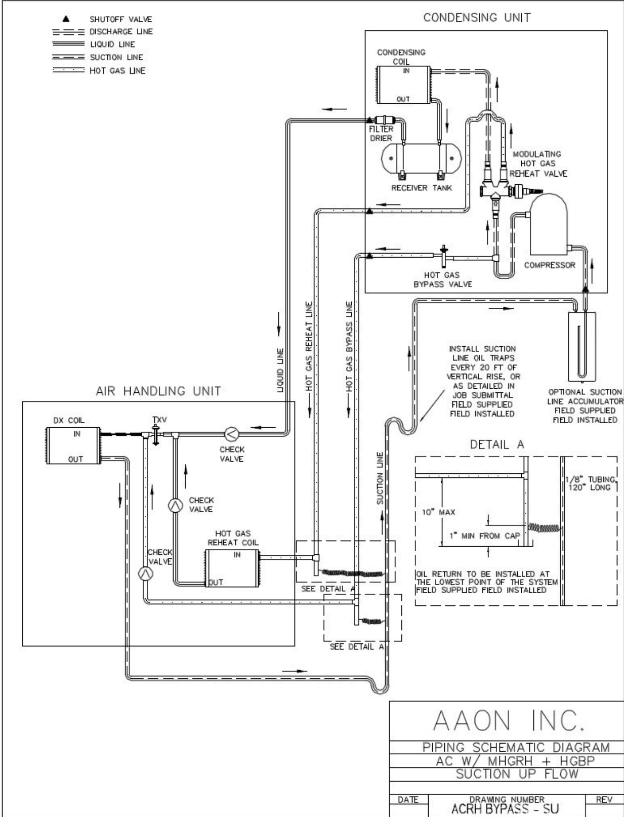
Figure 30 - A/C with Modulating Hot Gas Reheat and Hot Gas Bypass Split System Piping, Suction Up
