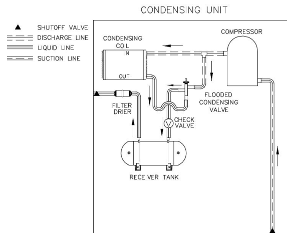
Figure 8 - LAC Piping Example
