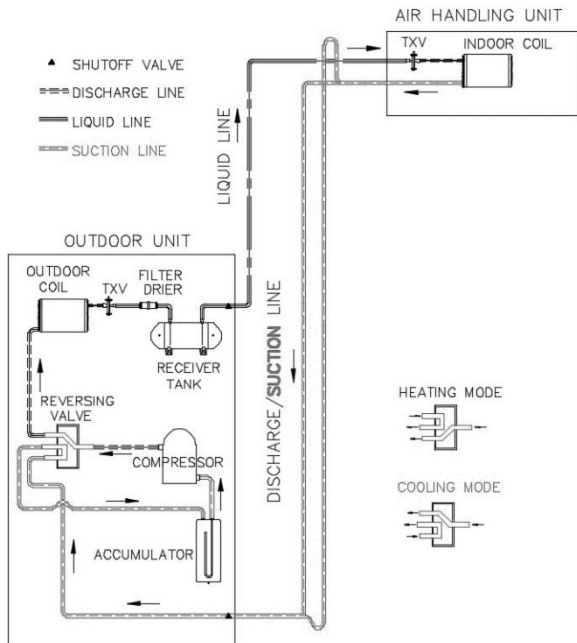
Figure 10 - Heat Pump Piping Schematic of Cooling Mode in Double Riser
