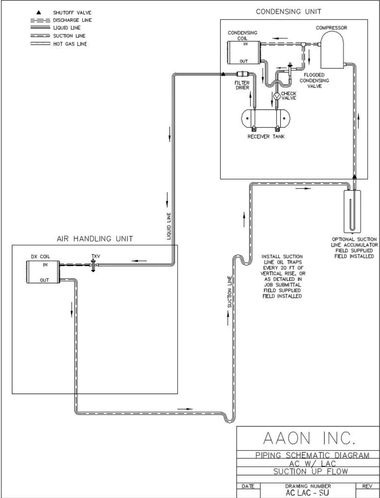
Figure 20 - A/C with LAC Split System Piping, Suction Up
