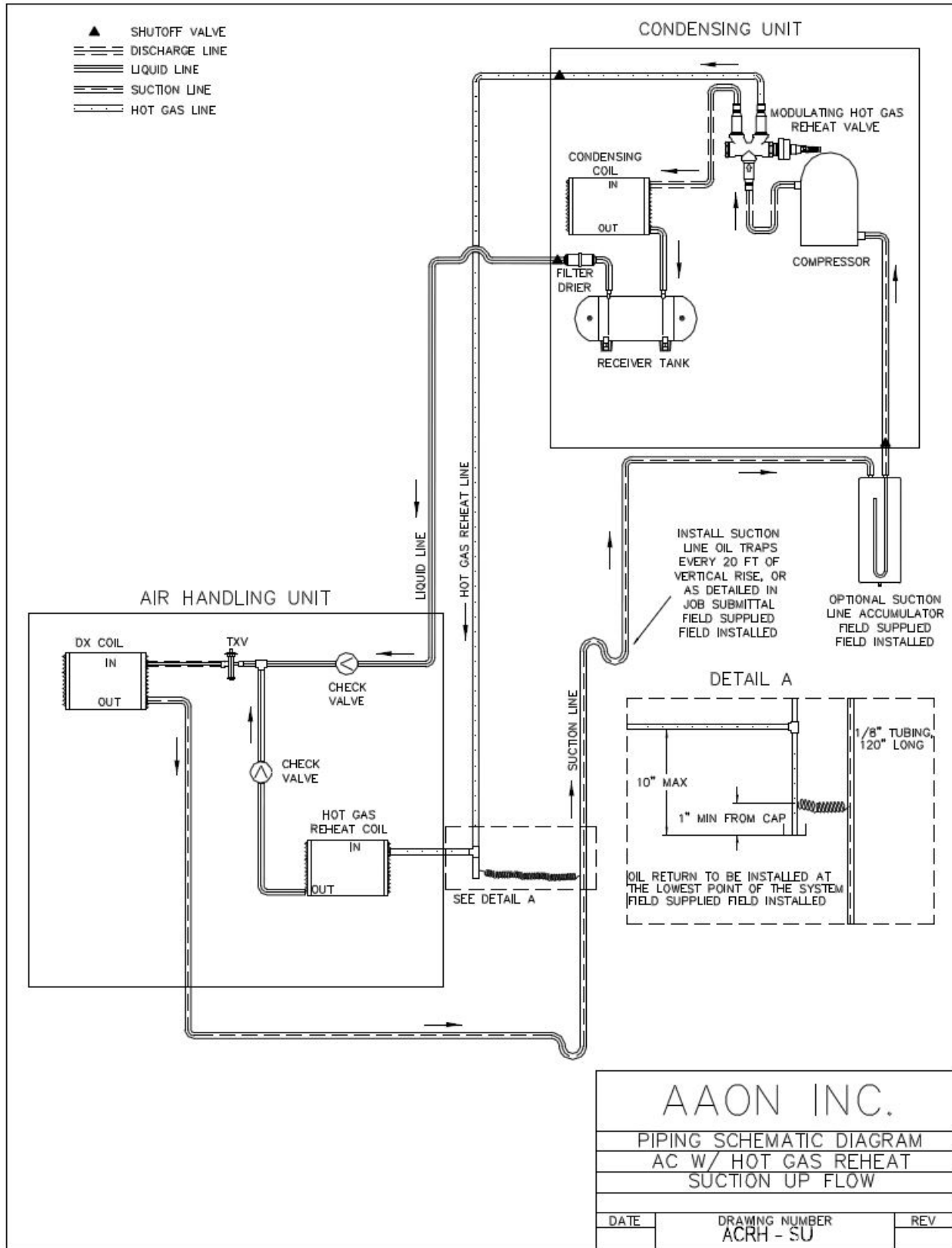
Figure 22 - A/C with Modulating Hot Gas Reheat Split System Piping, Suction Up
