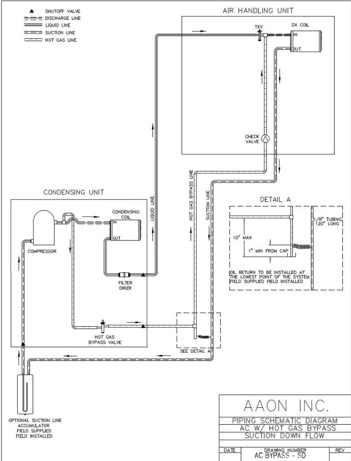
Figure 25 - A/C with Hot Gas Bypass Split System Piping, Suction Down
