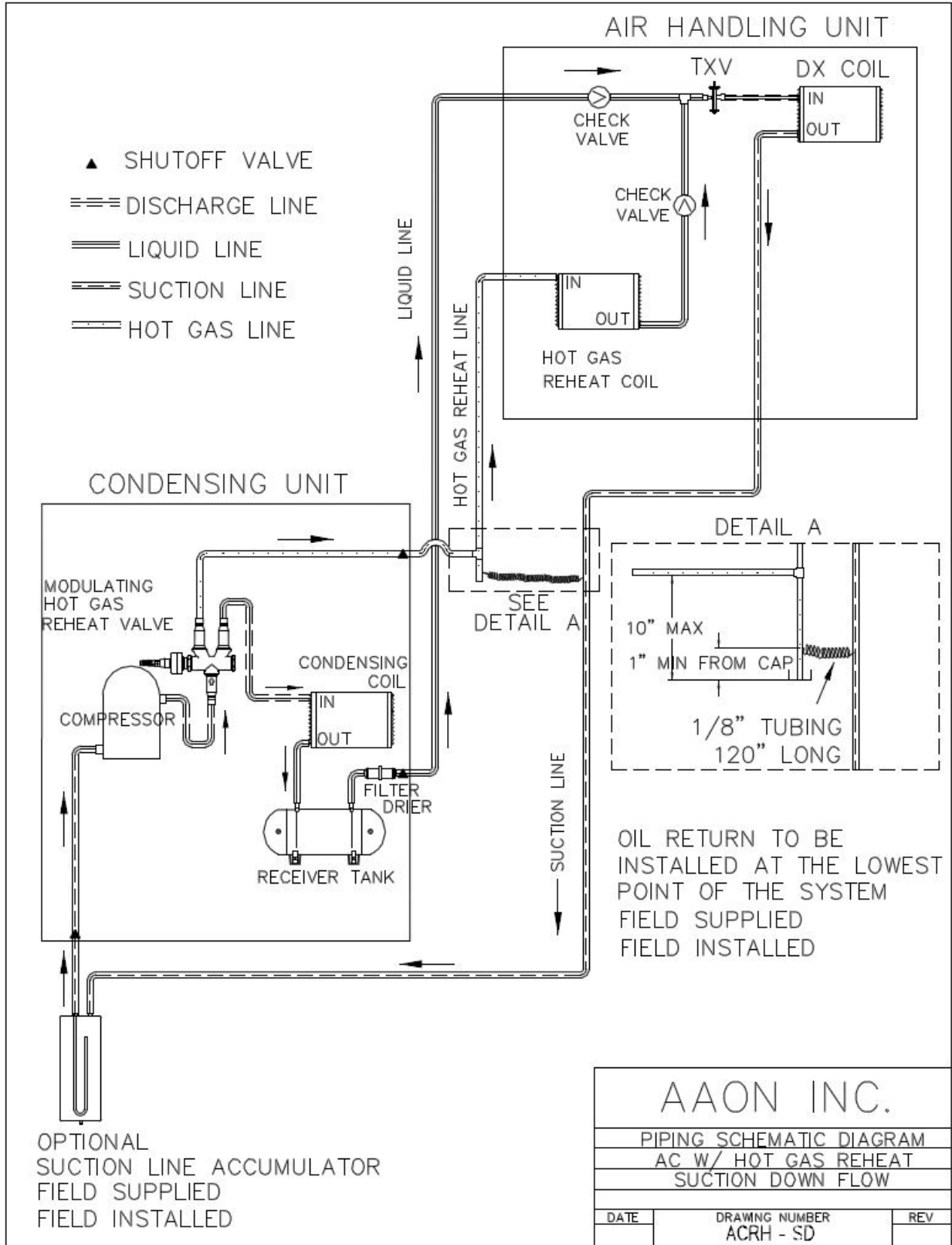
Figure 21 - A/C with Modulating Hot Gas Reheat Split System Piping, Suction Down
