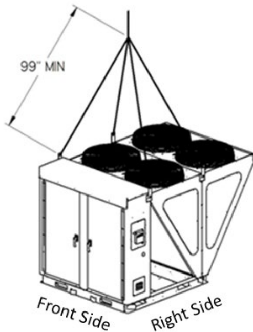
Figure 3 - Lifting Details and Orientation of a CF Series 9-70 ton Condensing Unit
