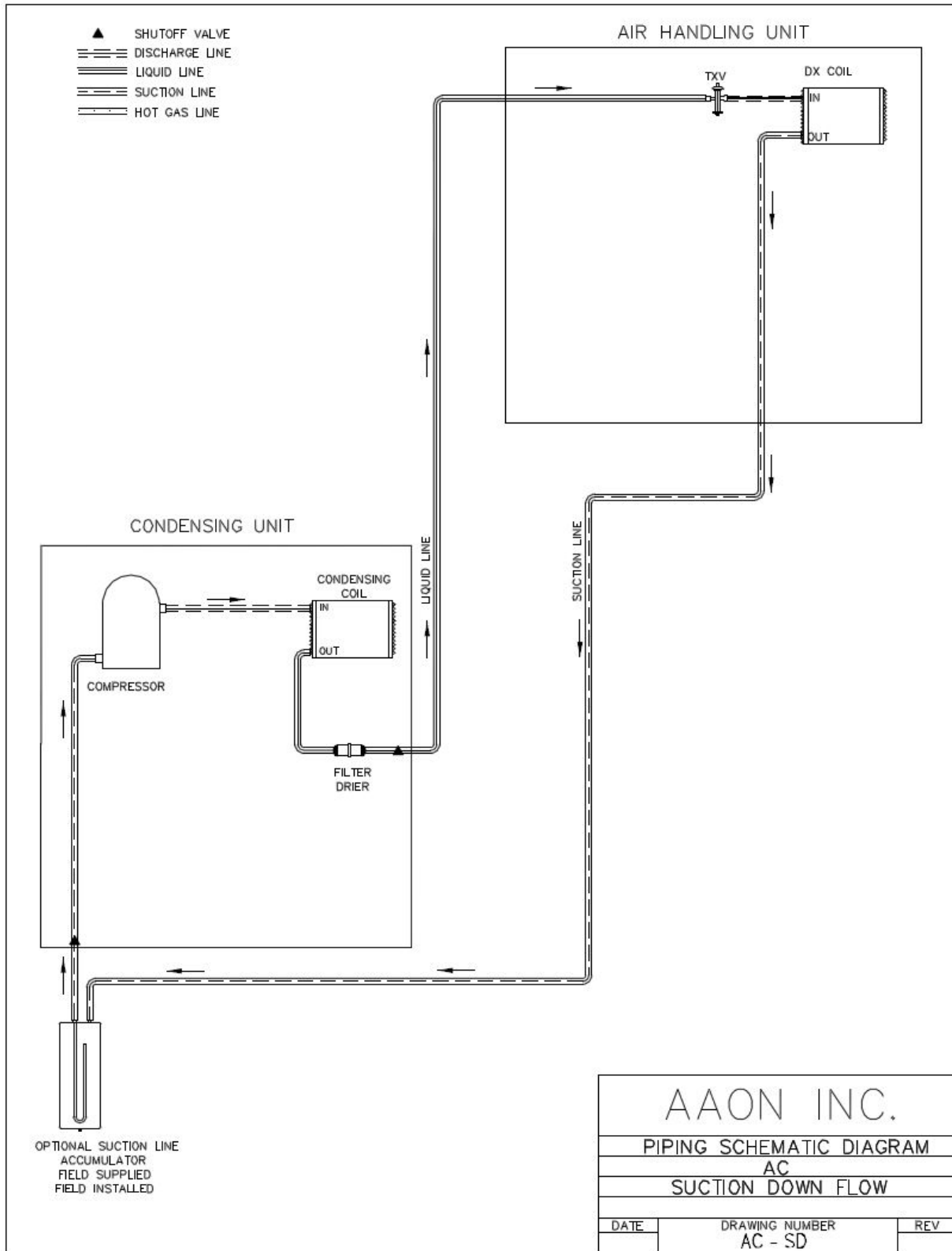
Figure 17 - A/C Split System Piping, Suction Down
