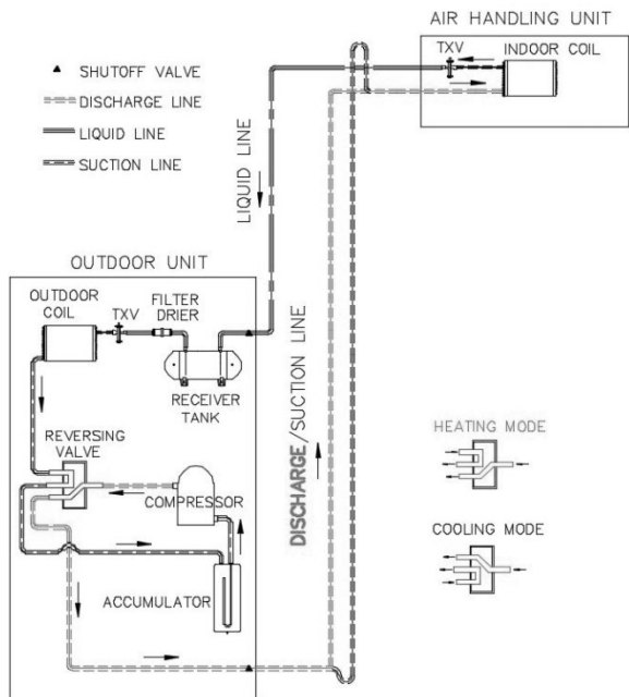
Figure 11 - Heat Pump Piping Schematic of Heating Mode in Double Riser
