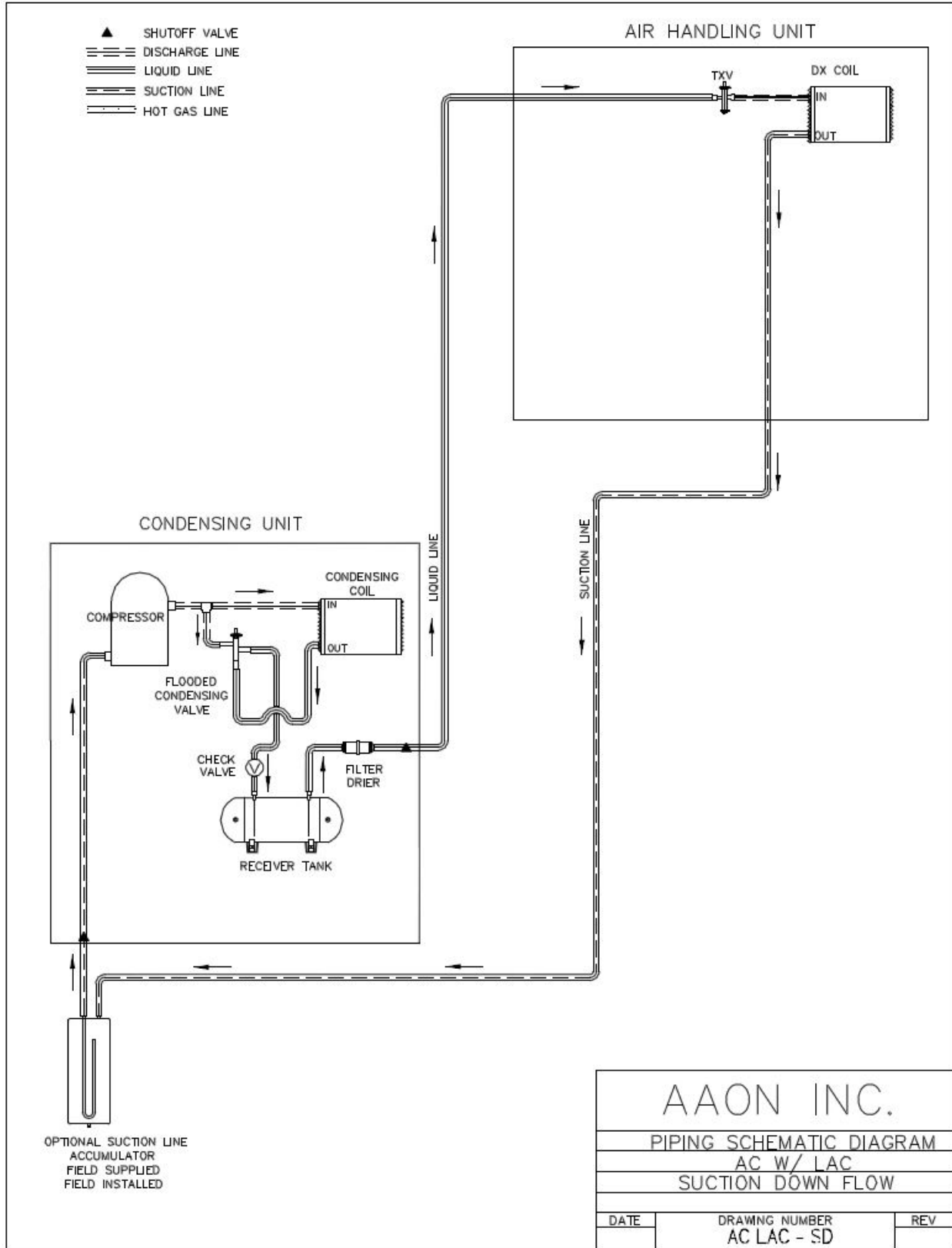
Figure 19 - A/C with LAC Split System Piping, Suction Down
