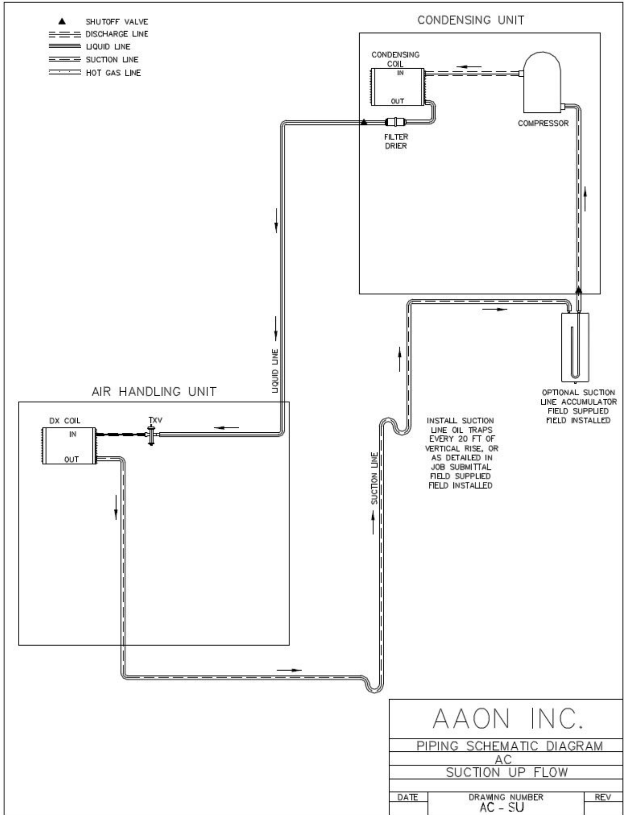
Figure 18 - A/C Split System Piping, Suction Up
