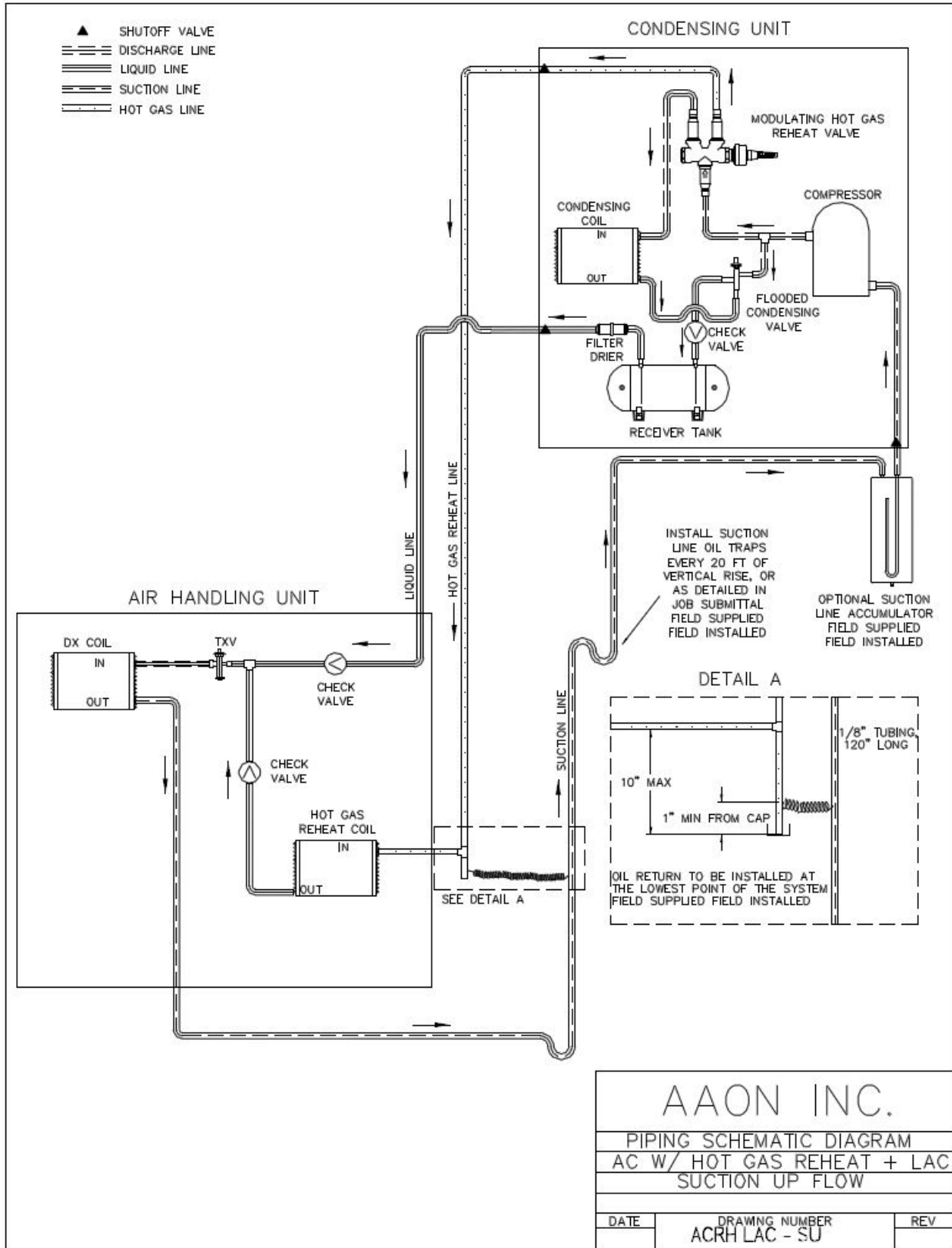
Figure 24 - A/C with Modulating Hot Gas Reheat Split + LAC System Piping, Suction Up
