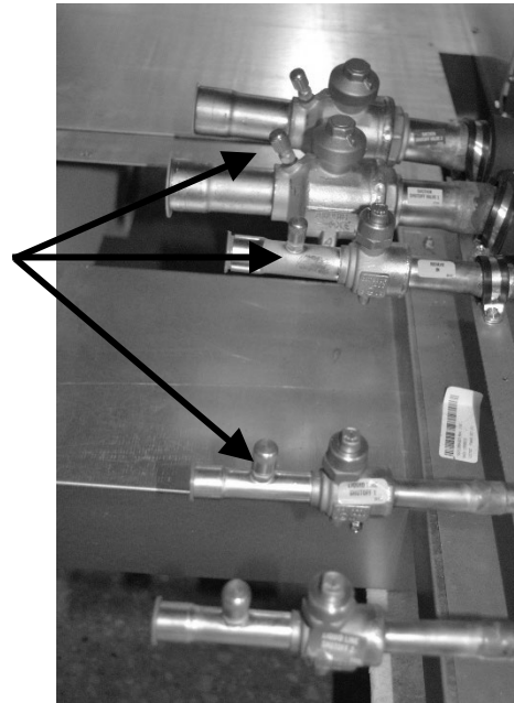
Figure 6 - CU evacuation connections
