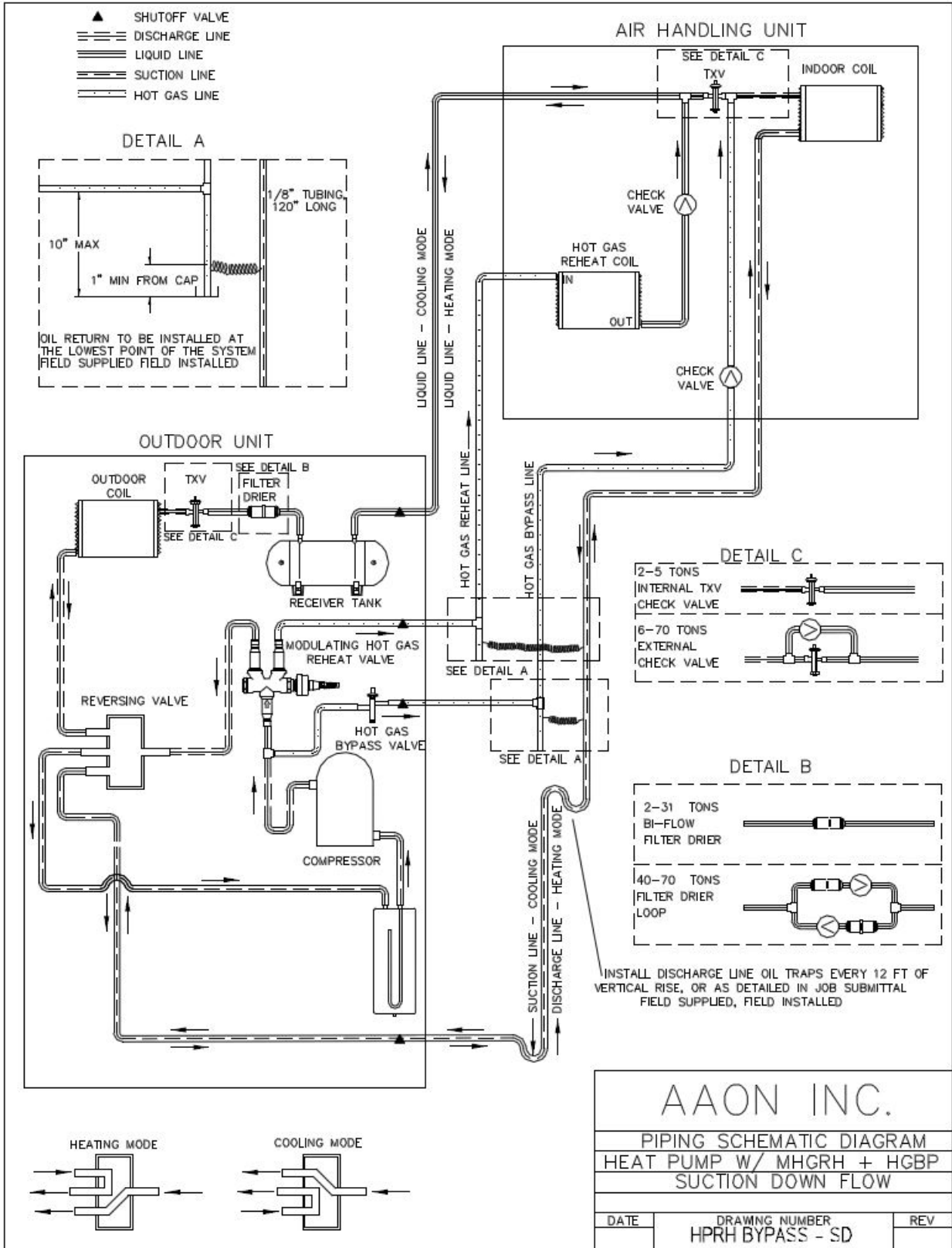
Figure 39 - Heat Pump with Modulating Hot Gas Reheat and Hot Gas Bypass Split System Piping, Suction Down
