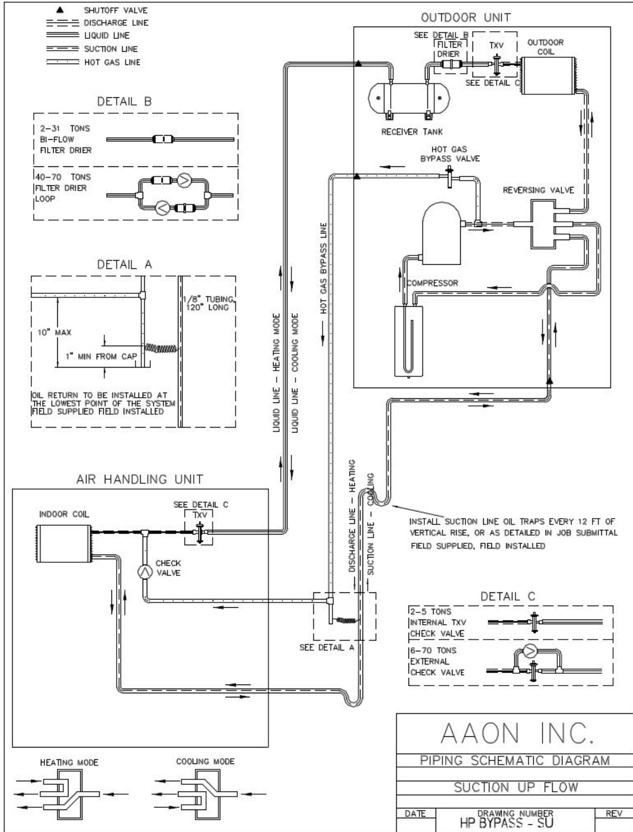
Figure 38 - Heat Pump with Hot Gas Bypass Split System Piping, Suction Up
