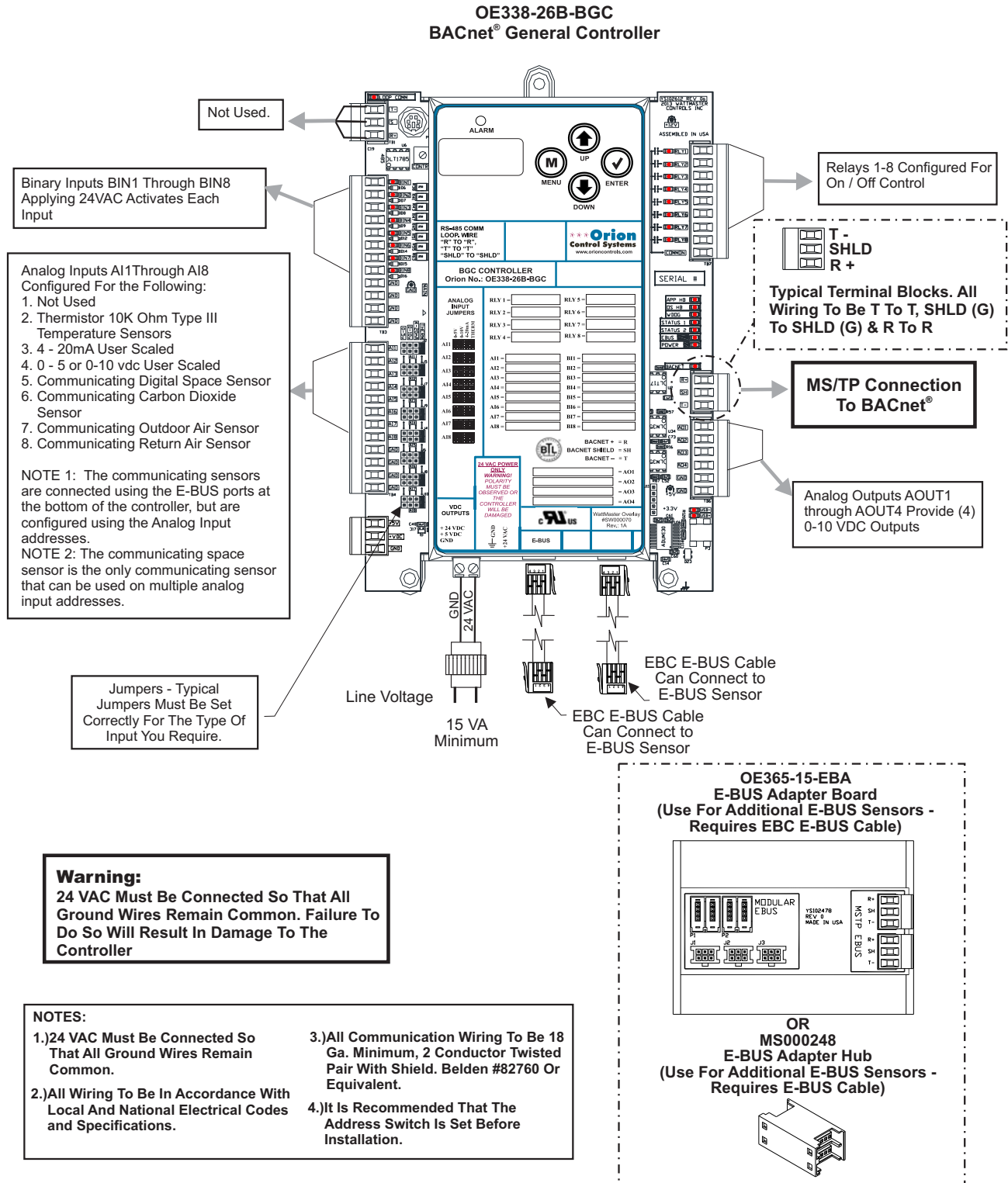
Figure 2: BGC Wiring Diagram
