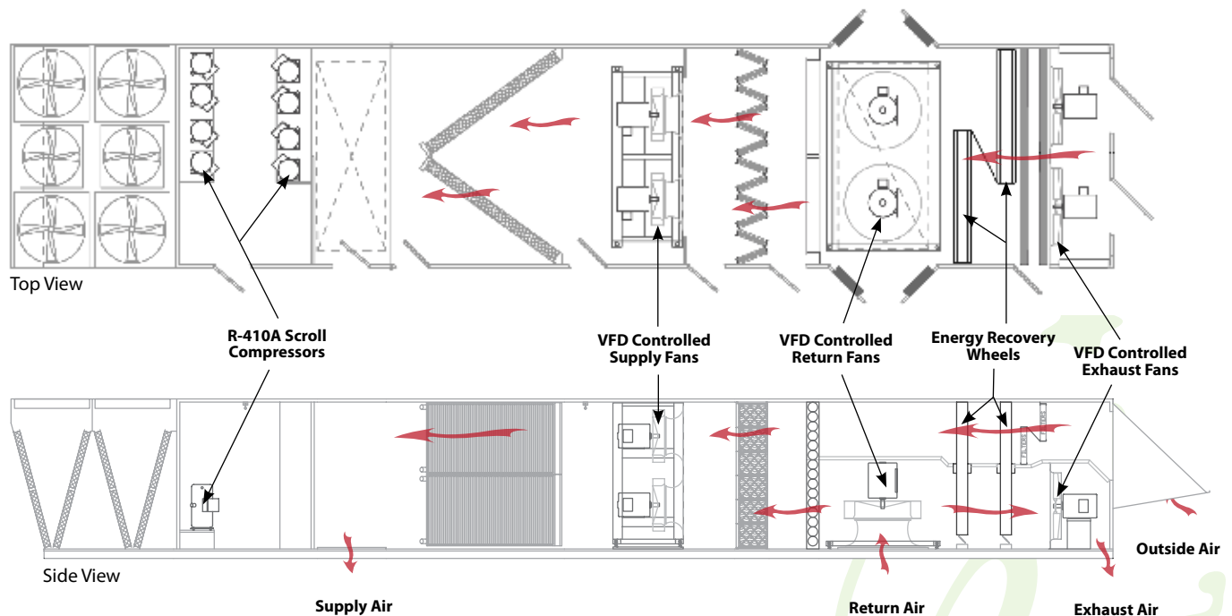
210 Ton AAONAIRE RL Series Unit, Energy Recovery Wheel with Power Return and Power Exhaust
